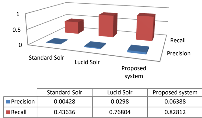
Fig.10: Precision (P) and Recall (R) for: Standard Inverted Index System (Standard Solr); Semantic Based Search System (Luicid Solr); and the Proposed Recommender System
